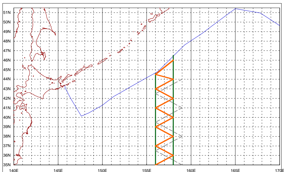
Fig 1. Survey area and the planned track lines. Orange thick line and broken gray line represented the track lines of KK1 and whale sampling line, respectively.
