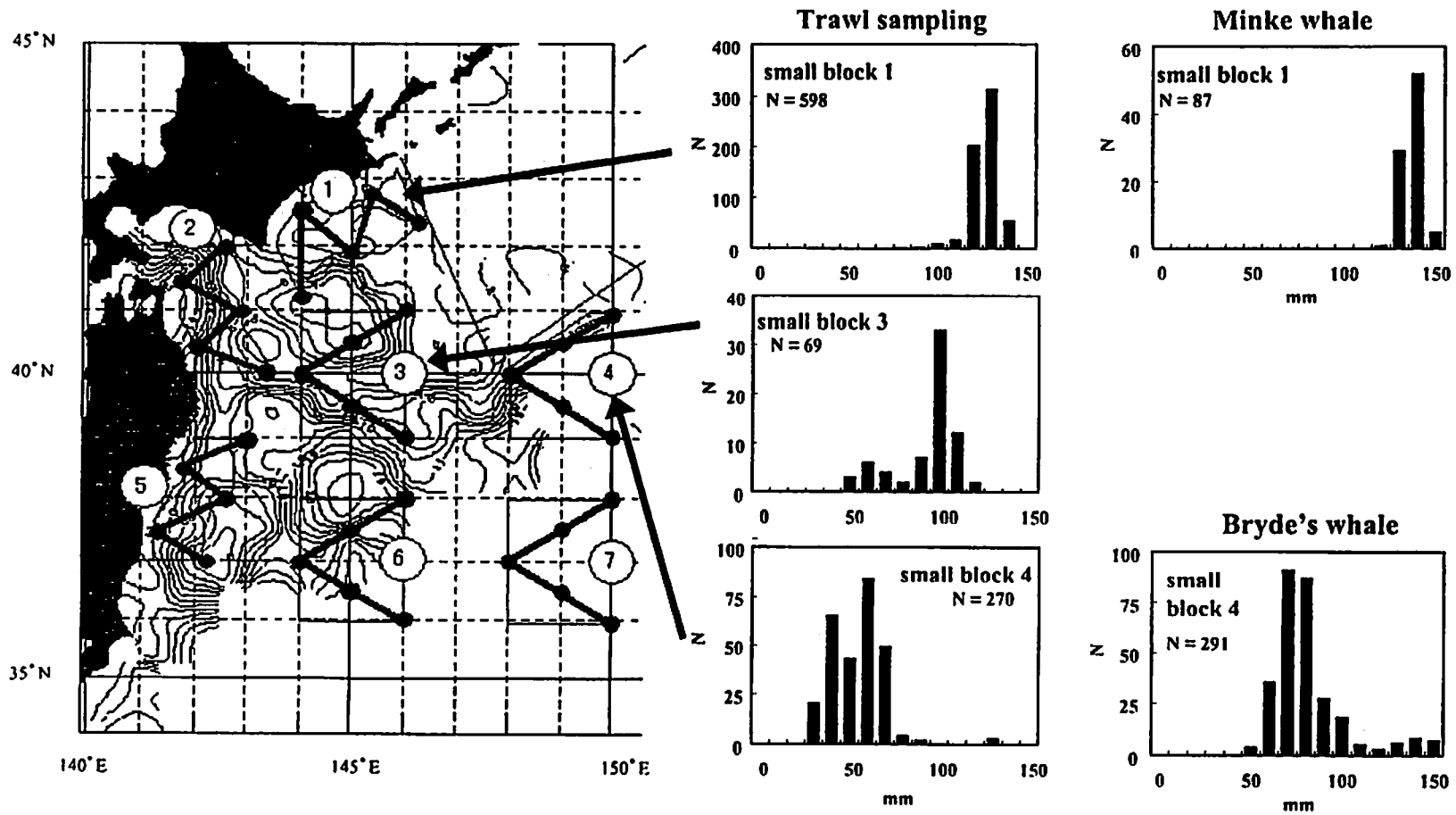
Fig. 18. Comparison of length frequencies of Japanese anchovies collected by trawling and from stomach contents of common minke and Bryde's whales in each small block.
