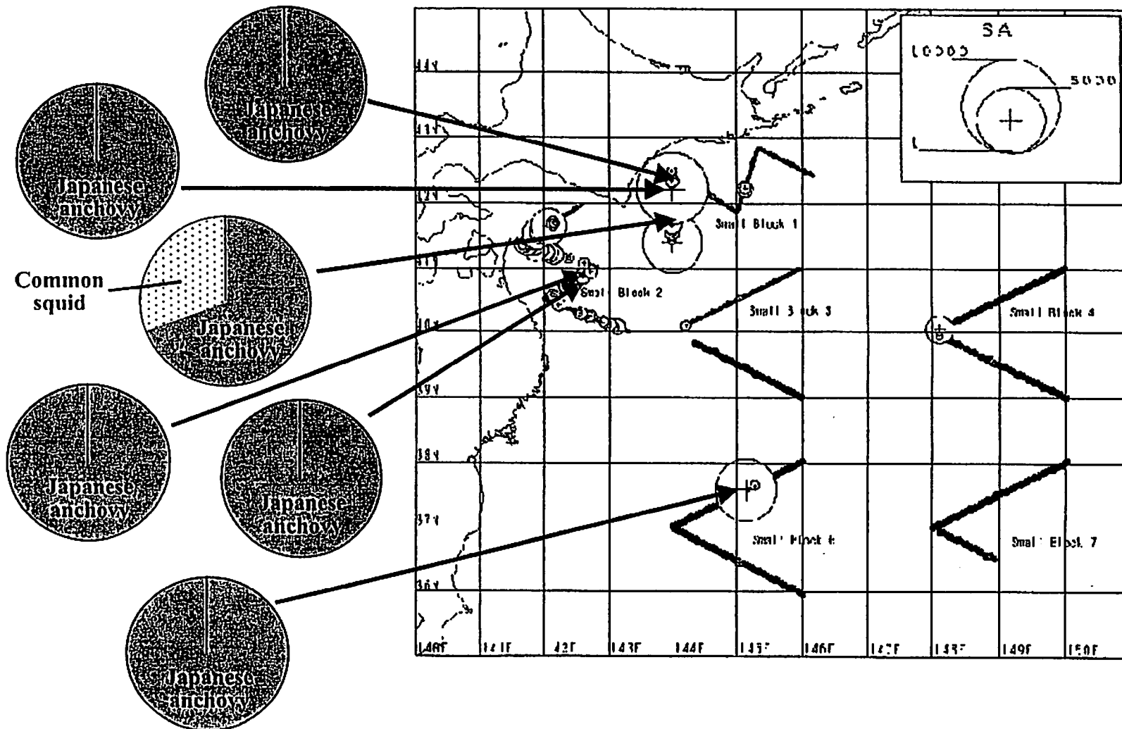
Fig. 6. Distribution of Japanese anchovy as suggested by the results of echo-sounder and trawl survey in JARPN II 2000.
