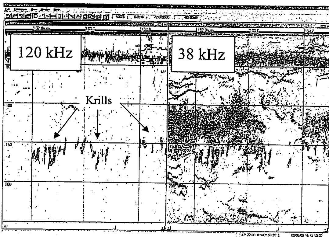
Fig. 3. The difference of marks of krills between 120 kHz and 38 kHz.
