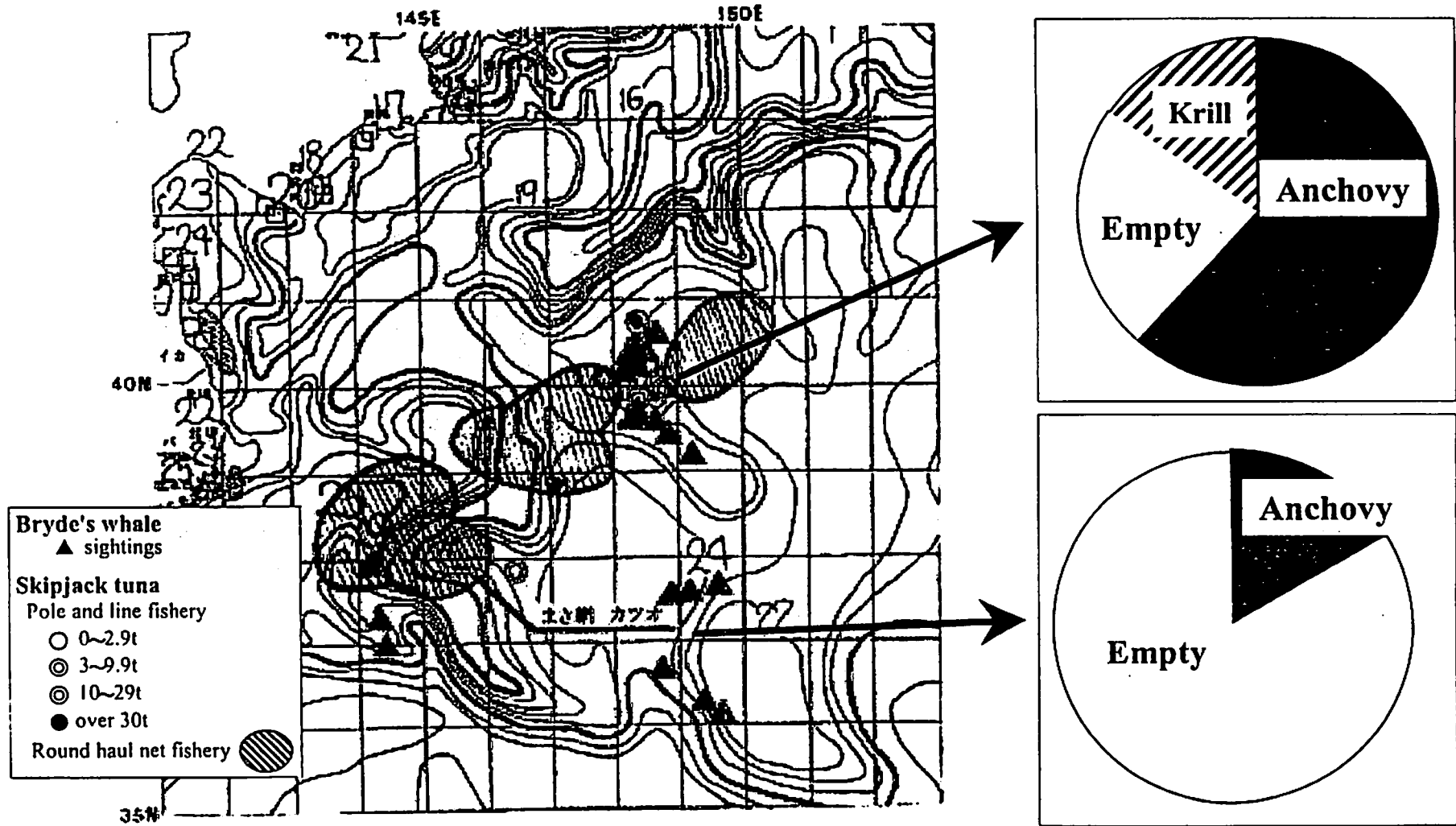
Fig. 19. Distribution of Bryde's whales and fishing grounds of skipjack tuna and the stomach contents of Bryde's whales.
