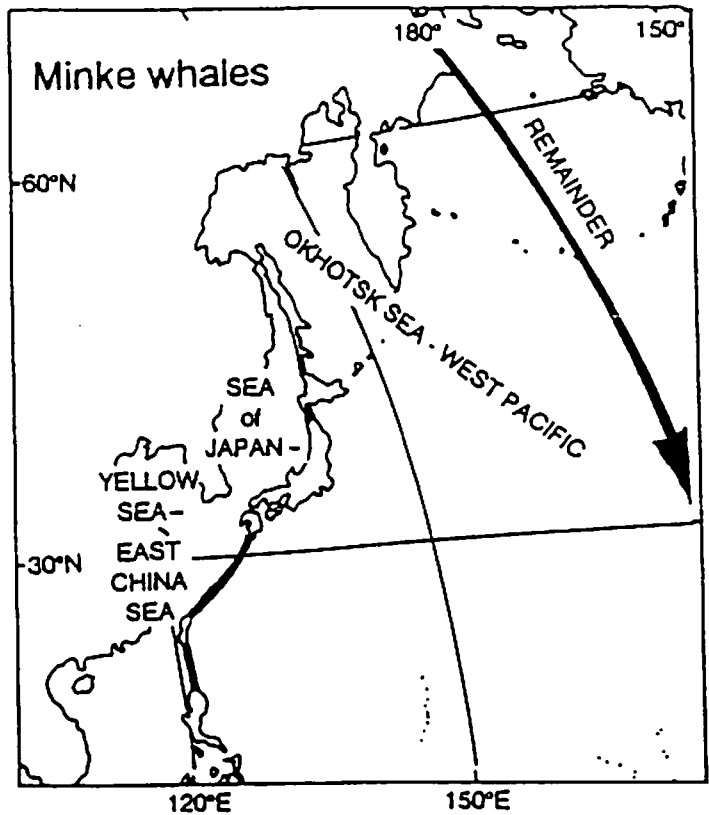
Fig. 2: Stock boundaries for the North Pacific minke whale adopted by the IWC in 1982 (IWC, 1983).
